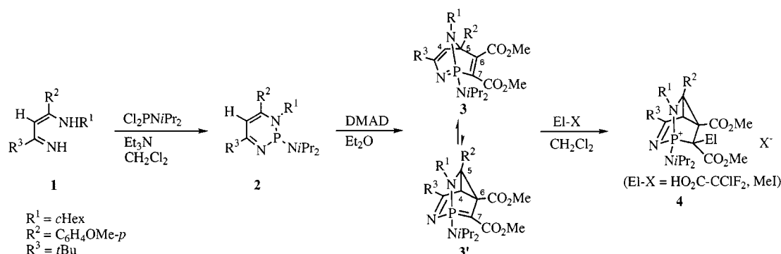
Scheme 1. Formation of heterocycles 3 by [5+2] Cycloaddition of diazaphosphinines 2 with dimethyl acetylenedicarboxylate and their reaction with electrophiles
