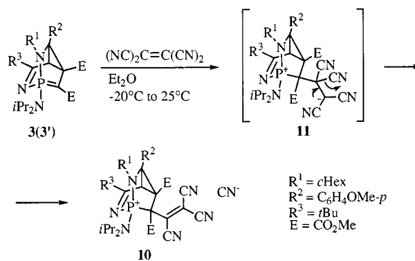
Scheme 5. Formation of phosphonium salt 10 from 3 and tetracyanoethylene
