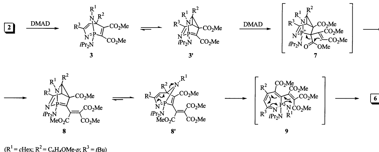
Scheme 4. Mechanistic proposal for the formation of diazaphosphaazulene derivatives 6
