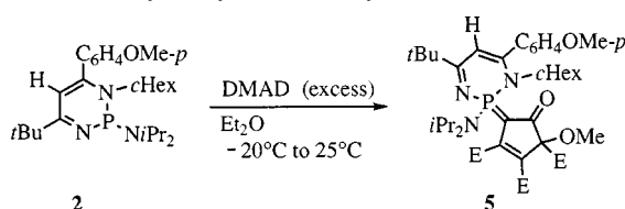
Scheme 2. Formation of diazaphosphinine derivative 5 from 2 and dimethyl acetylenedicarboxylate
