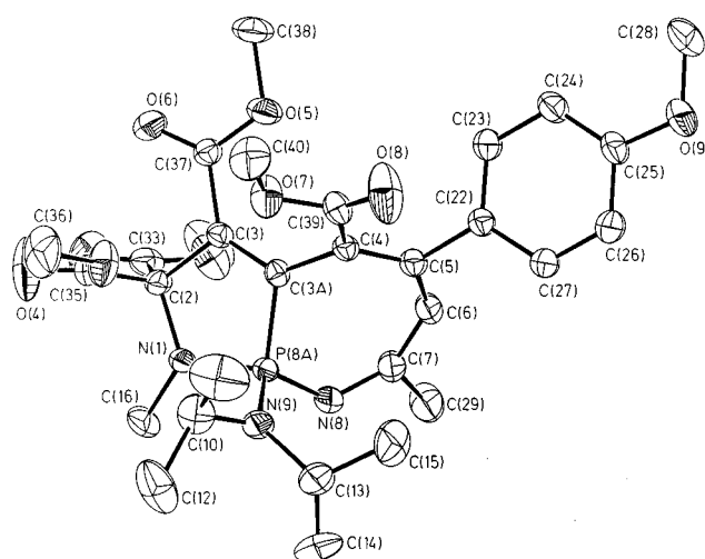
Figure 1. Crystal structure of 6a [a]
