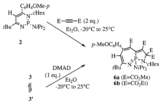
Scheme 3. Formation of diazaphosphaazulene derivatives 6 from 2 or 3 and acetylenedicarboxylic acid esters
